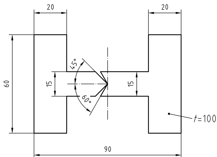
Figure C.1 — Dimensions of the hinge for beam type A ( d < 16 mm)
